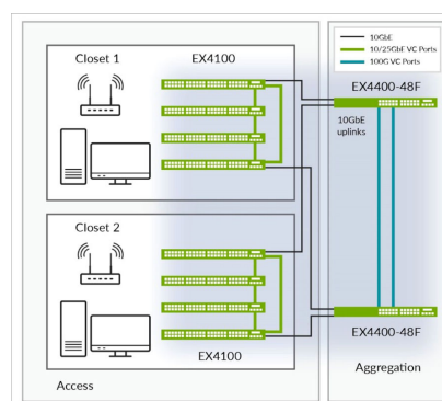
Figure 1: EX4100-H Virtual Chassis configuration interconnected via dedicated front-panel 25GbE ports
